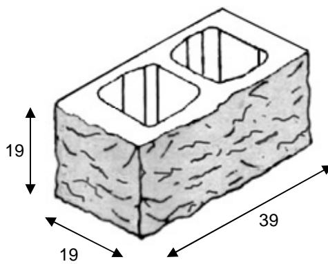
SPLIT Esquina 1 Cara Lisa 39 x 19 x 19
