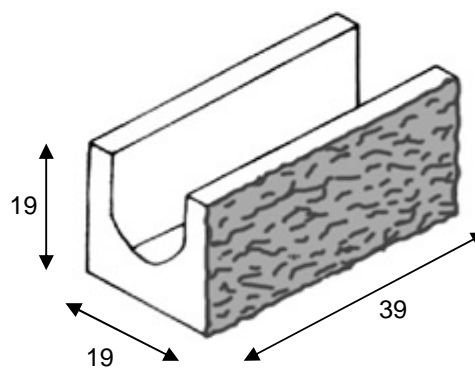
Zuncho SPLIT 39 x 19 x 19
